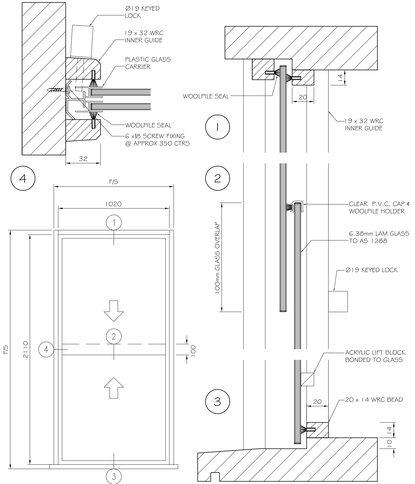
ELEVATION SCALE 1:10
